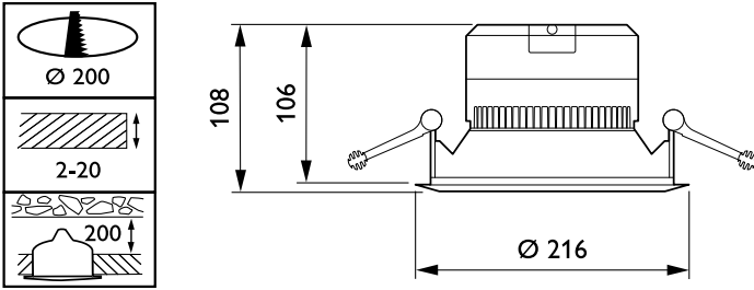
DN140B LED20S/840 PSU C IP54 P16
