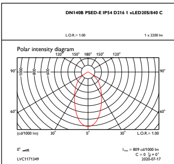
OFPC1_DN140BPSED-EIP54D2161xLED20S840C
