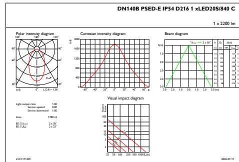
IFAS1_DN140BPSED-EIP54D2161xLED20S840C
