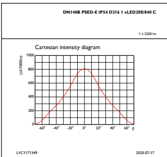
IFCC1_DN140BPSED-EIP54D2161xLED20S840C
