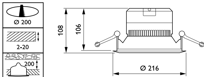
DN140B LED20S/830 PSU C P16
