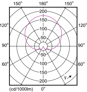
CorePro LEDbulb ND 13-100W A60 830
