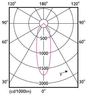
Downlight RS061B G2 LDNR 827 WH TW-LDD
