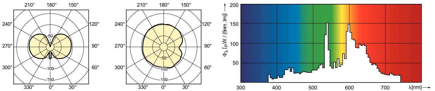
LLDL_CDM-T-E_0001-Light distribution diagram
