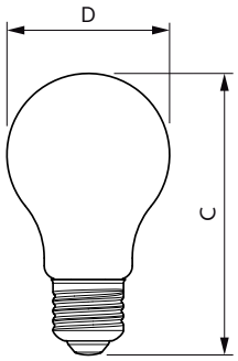
MASTER VLE LEDBulbDT10.5-100W E27 927A60CLG
