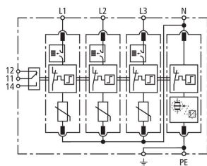
Basic circuit diagram DG M TT ACI 275 FM
