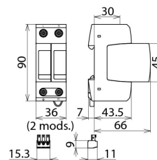
Dimension drawing DG M TN 275 FM
