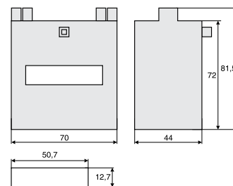
Z-MG/WAS-800, -1000
