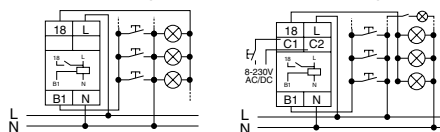
3-draads schakeling (TLE) 4-draads schakeling (TLK)
