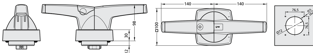
Type K5D
