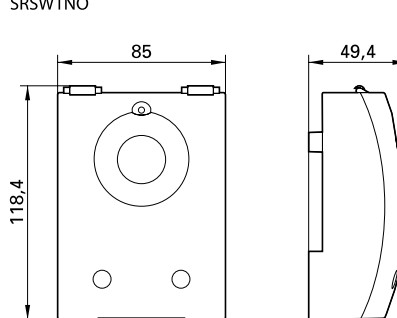
SRSW1NO
