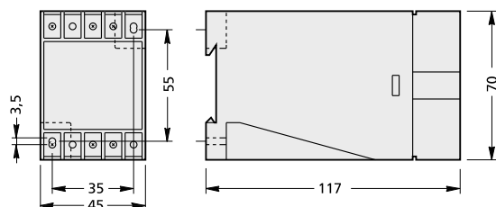
Type ELM 25
