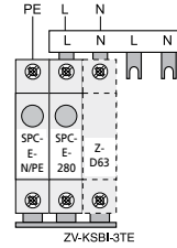
TN-S/TT-System 3 x 240/415 VAC 3 x 230/400 VAC 3 x 220/380 VAC
