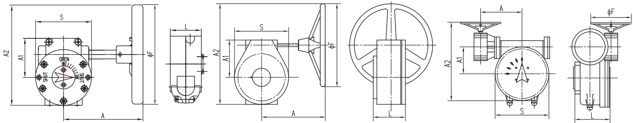
Single-stage Worm Gear ZD6N-S100 ~ ZD6N-S350
