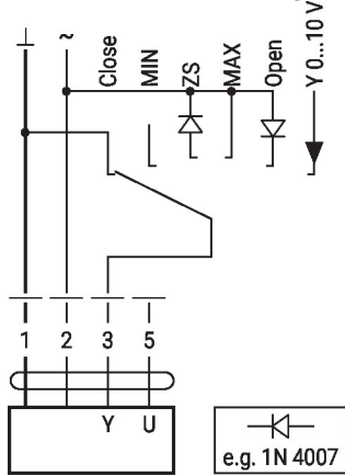
Override control and limiting with AC 24 V with rotary switch
