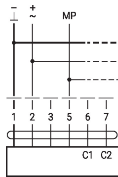
MP-Bus, supply via 3-wire connection
