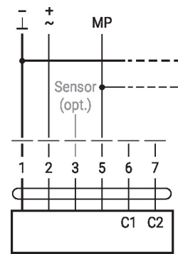
MP-Bus via 2-wire connection, local power supply
