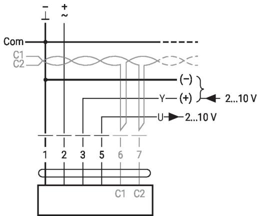
BACnet MS/TP / Modbus RTU with analogue setpoint (hybrid mode)
