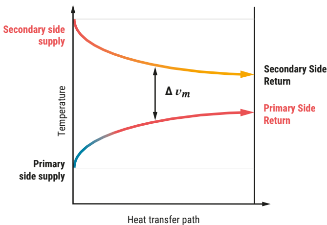
Abb. 63: \Delta\theta_m average differential temperature for direct flow.
