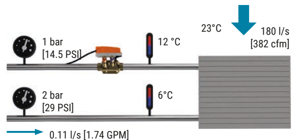
Abb. 78: FCU at design operation.
