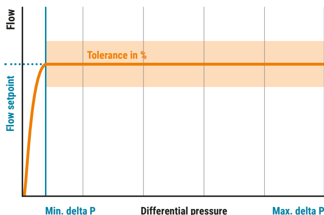
Abb. 85: Dynamic balancing of a chilled beam.
