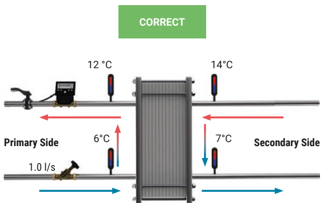
Abb. 66: Typical design flow (cooling application).
