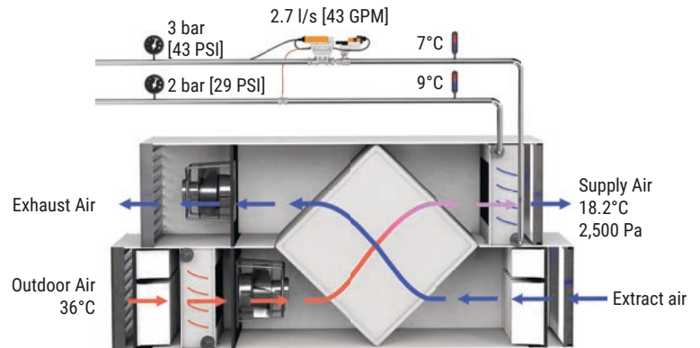
Abb. 56: AHU without valve overflow.
