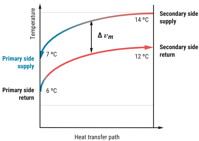
Abb. 67: \Delta\vartheta_m average differential temperature with design flow.
