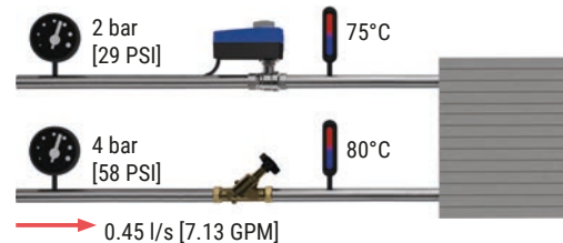
Abb. 98: FCU heating mode and differential pressure increase.
