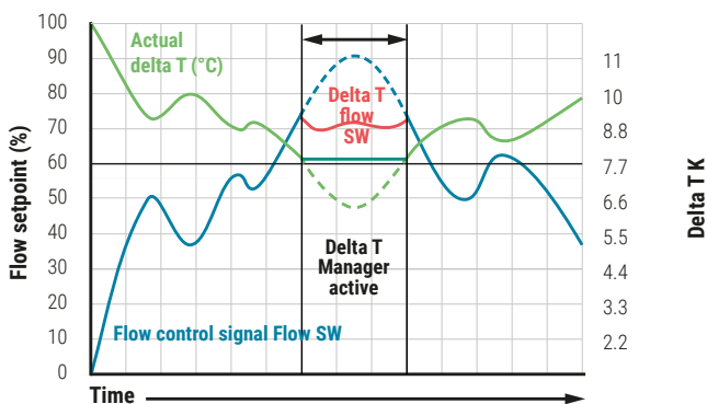
Abb. 32: 'Scaling delta T manager' scales the delta T setpoint, depending on the current flow rate.
