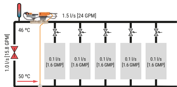
Abb. 105: With an Energy Valve, not only leaking short-stroke globe valves but also an open bypass can be clearly identified.
