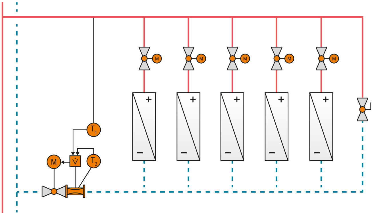
Abb. 101: A schematic diagram of the installation of an Energy Valve in a branch.
