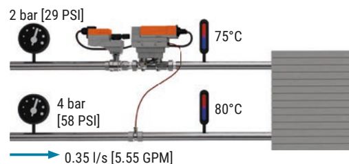
Abb. 99: FCU in cooling mode, using a pressure-independent EV.
