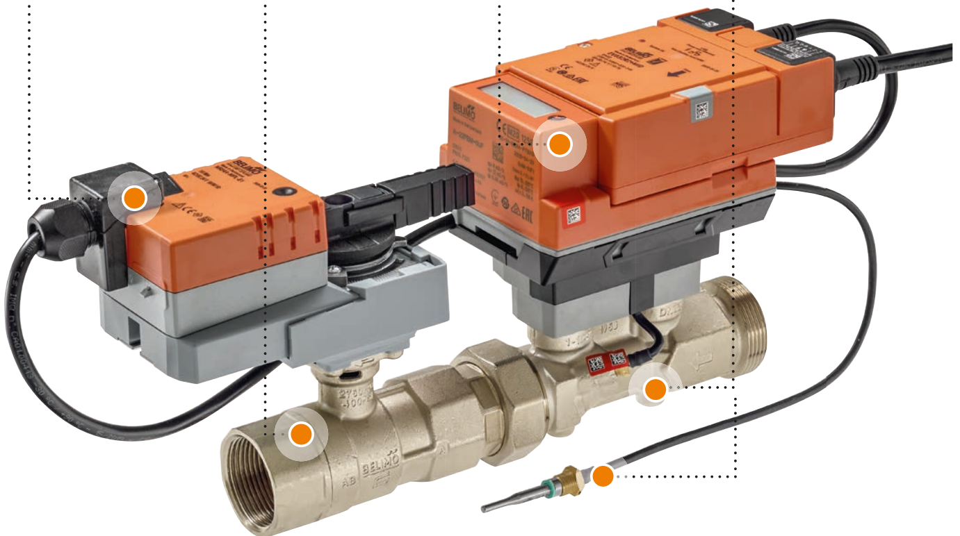
Abb. 21: The components of the Belimo Energy Valve™.
