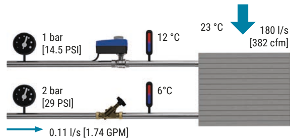
Abb. 76: FCU at design operation.
