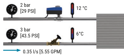
Abb. 96: FCU in cooling mode.
