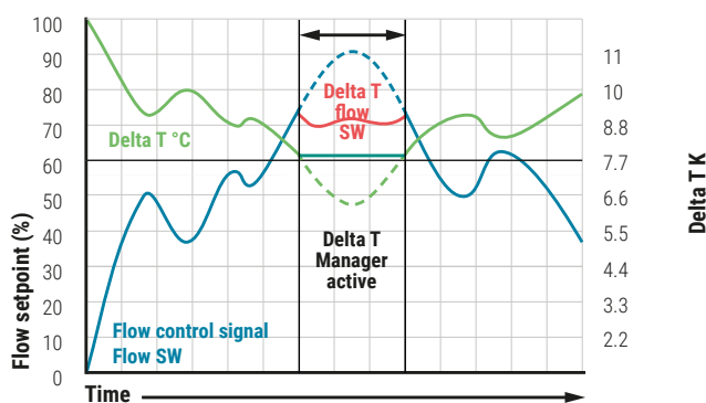
Abb. 30: The delta T manager detects a low delta T, becomes active, and reduces the flow to ensure the minimum delta T.
