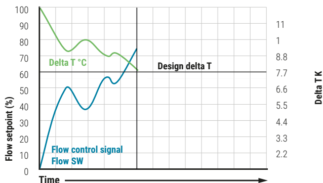
Abb. 28: When the demand increases and the flow changes, the actual delta T starts to decrease.
