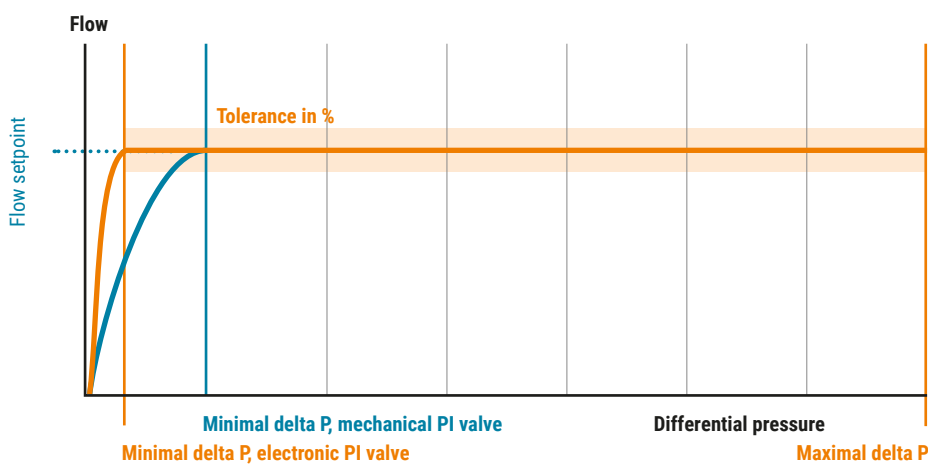
Abb. 13: Electronic PI valves can typically maintain the flow rate at lower delta P than can mechanical PI valves.
