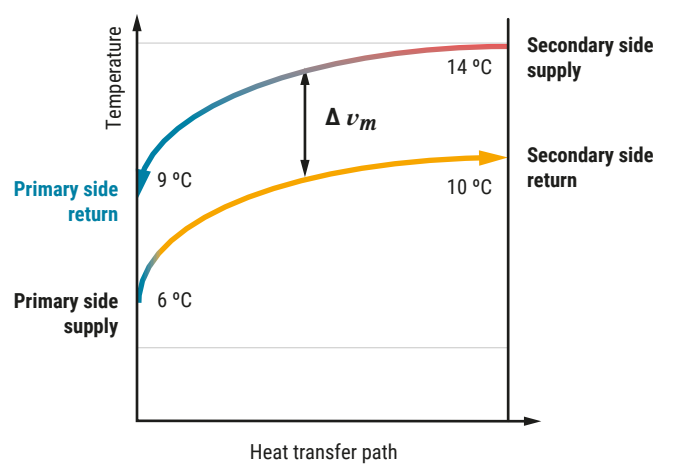
Abb. 69: \Delta\vartheta_m mean differential temperature with saturation.
