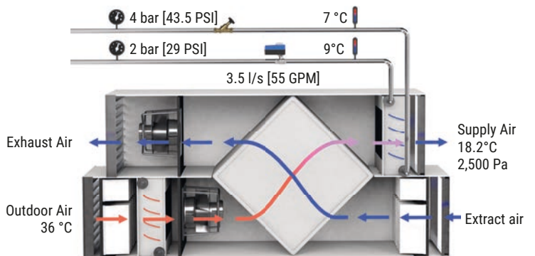
Abb. 54: AHU with valve overflowing.
