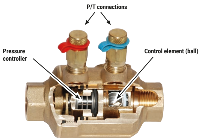
Abb. 9: Components of a mechanical PI valve, e.g. a PIQCV.
