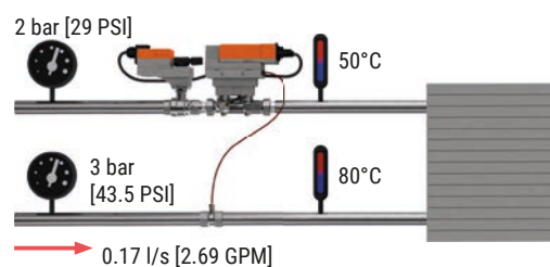
Abb. 100: FCU, with BMS-corrected heating setpoint and required flow rate.
