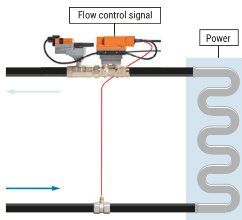
Abb. 25: Power control of the energy input to a consumer.
