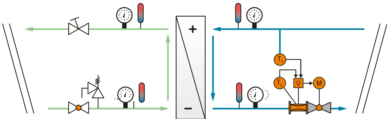
Abb. 61: Supply side (green) and consumer side (blue).
