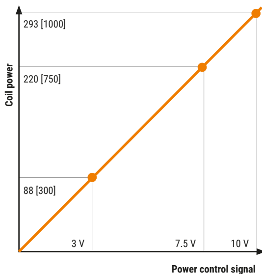
Abb. 27: Example of a coil using power control mode.
