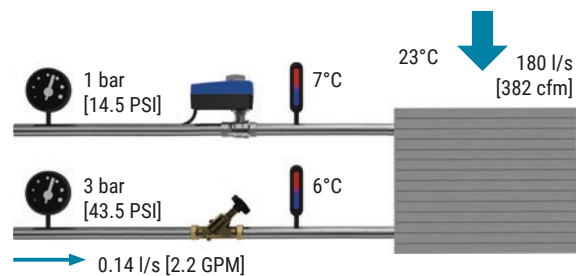
Abb. 77: FCU with valve overflowing.
