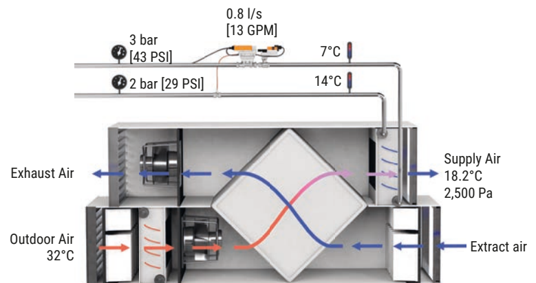
Abb. 57: AHU with delta-T-optimised flow rate.
