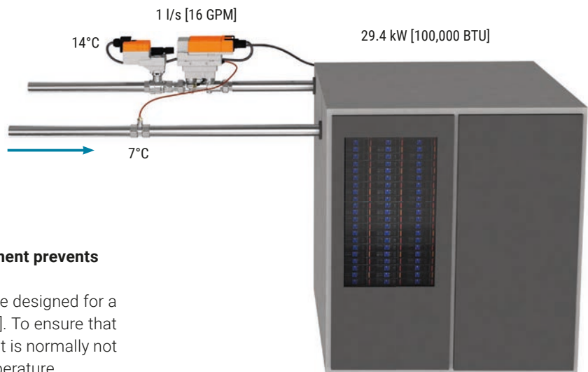
Abb. 111: CRAC device under "design load conditions".
