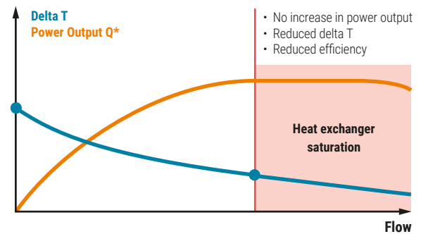
Abb. 106: Low delta T syndrome
