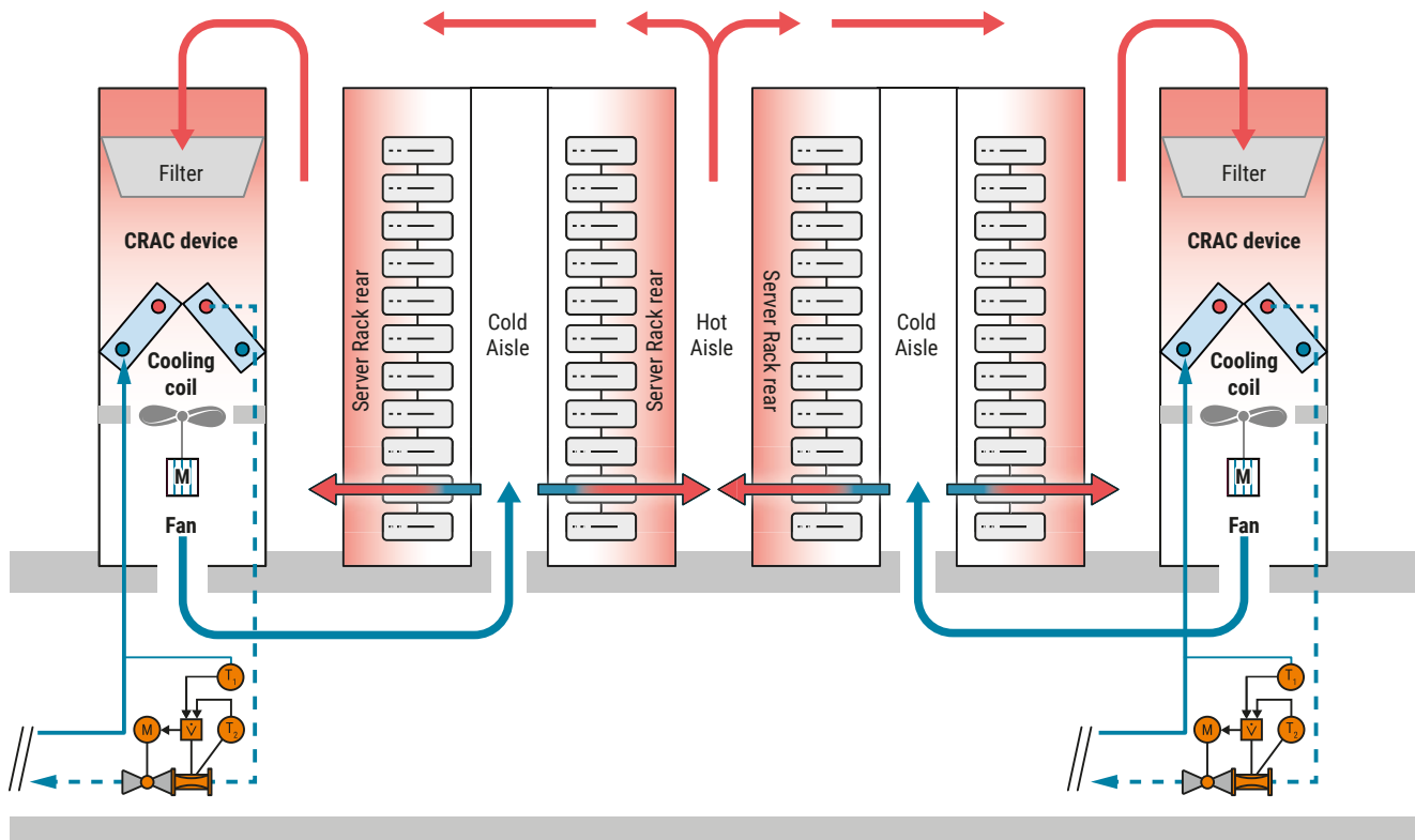
Abb. 110: Schematic of a CRAC device, including airflow to/from the racks.
