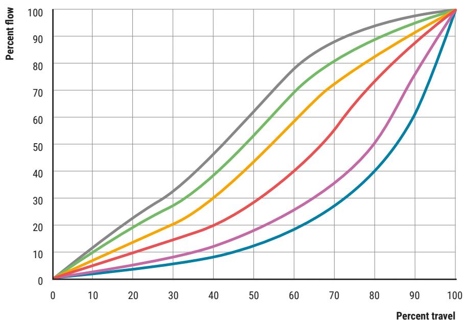
Abb. 22: The distortion of the characteristic curve that could occur if the valve is left in position control.
