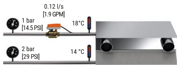
Abb. 90: Chilled beam with a mechanical PI valve.
