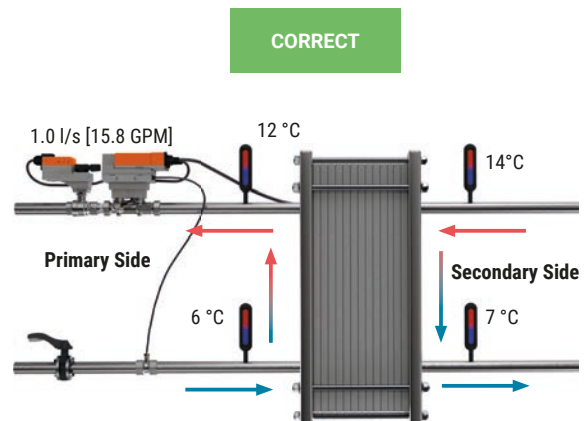
Abb. 71: Dynamic balancing with power characteristic monitoring.
