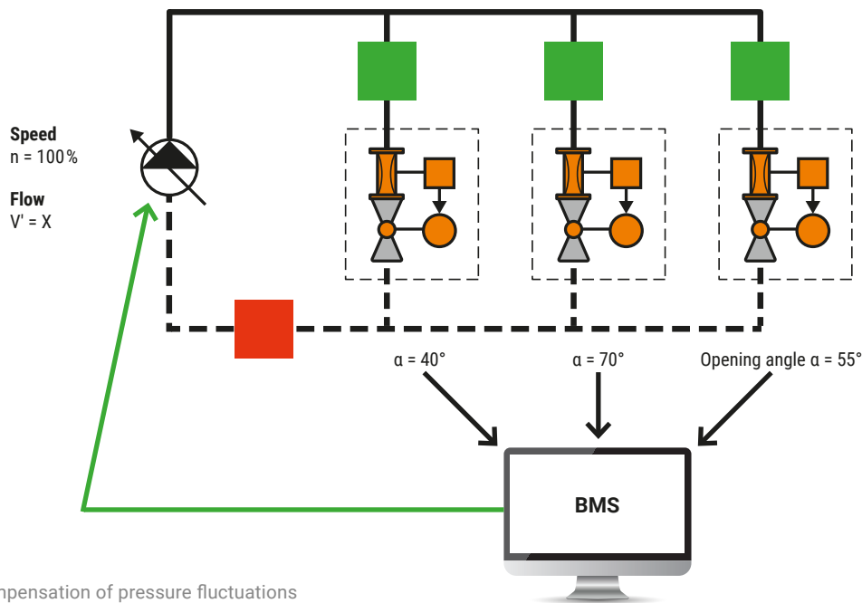
Abb. 16: Compensation of pressure fluctuations by changing the valve opening.
