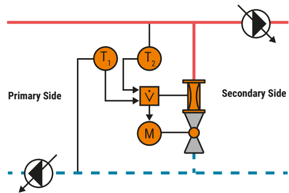
Abb. 47: An Energy Valve that monitors the temperature spread of the primary part and the flow via the hydronic deflector.
