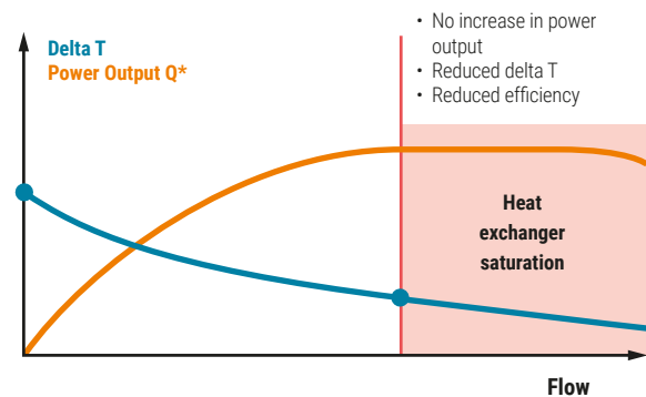
Abb. 51: Low delta T syndrome
