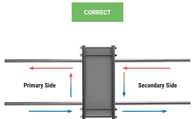
Abb. 64: Cooling transfer station connected in contraflow.
