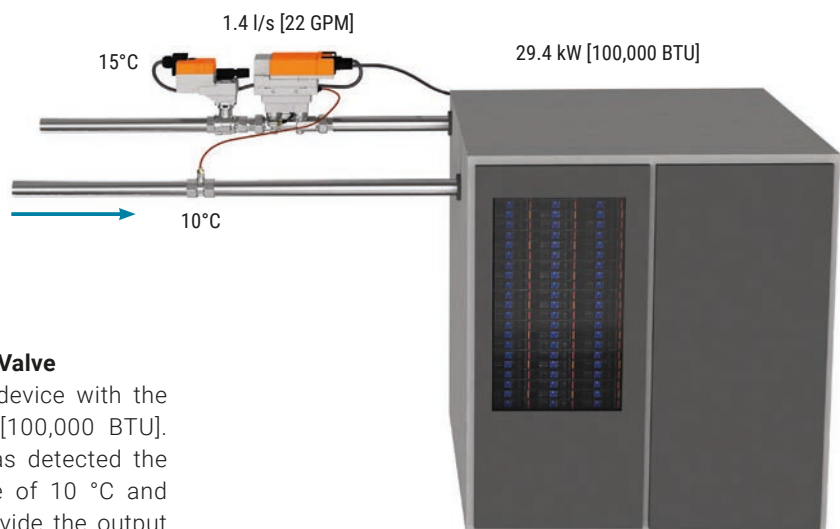
Abb. 112: CRAC device with higher supply temperature to save energy.
