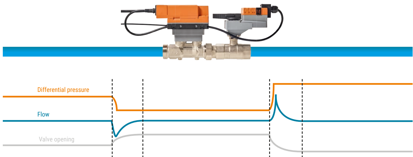
Abb. 15: Compensation of pressure fluctuations by changing the valve opening.
