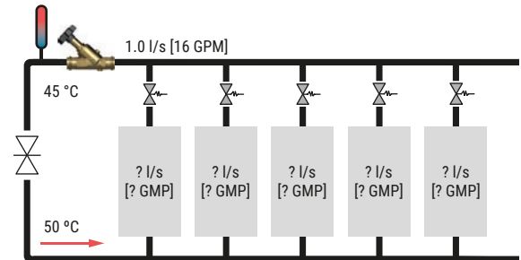
Abb. 102: Mechanical balancing valves allow only static balancing of the total flow, whereby the flow rates to each individual unit are unknown.
