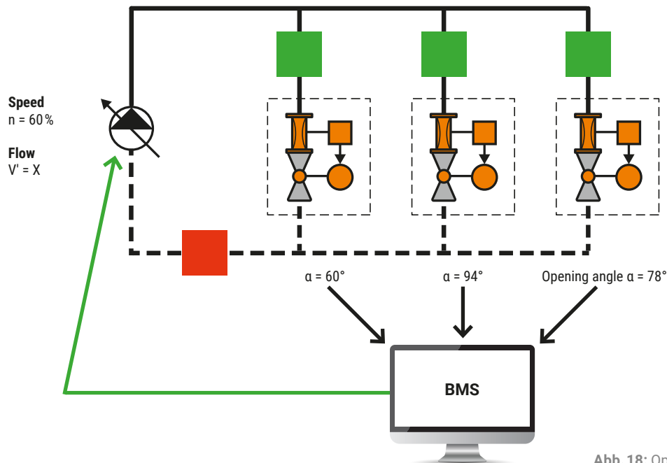
Abb. 18: Optimised operation
