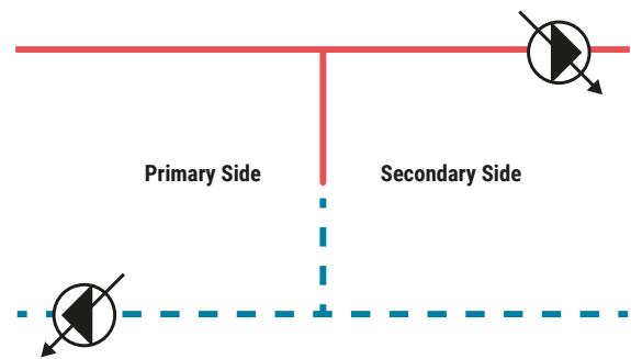
Abb. 46: Simple representation of a primary/secondary circuit with a hydronic deflector.
