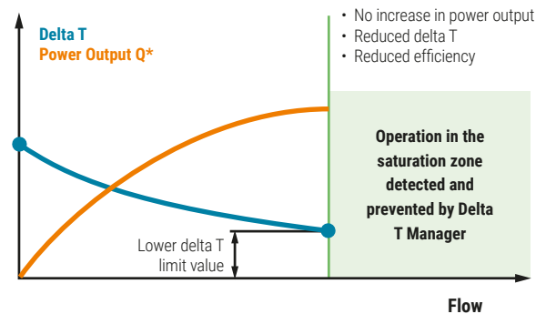
Abb. 52: Improved energy efficiency with the Energy Valve™ delta T manager enabled.
