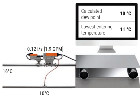
Abb. 92: Chilled beam with an Energy Valve, for which the BMS calculates the dew point using data from a room sensor.
