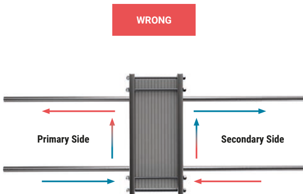
Abb. 62: Cooling transfer station connected in direct current.
