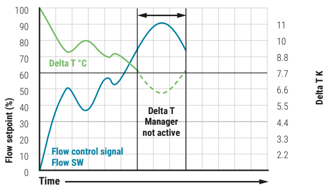
Abb. 29: If the delta T manager was not active, the flow setpoint drives the demand so high that the delta T falls below the desired setpoint of 7.7 K.
