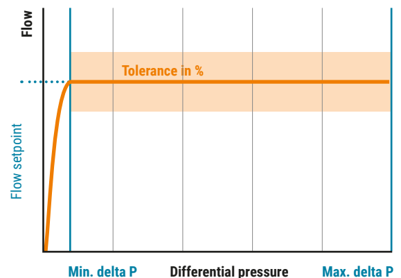
Abb. 24: Control characteristics in flow control mode.
