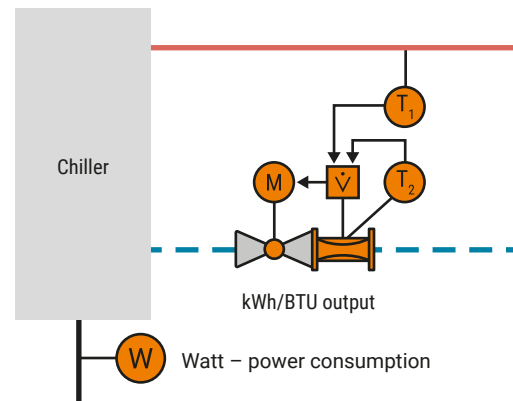
Abb. 120: Chiller with cooling circuit.
