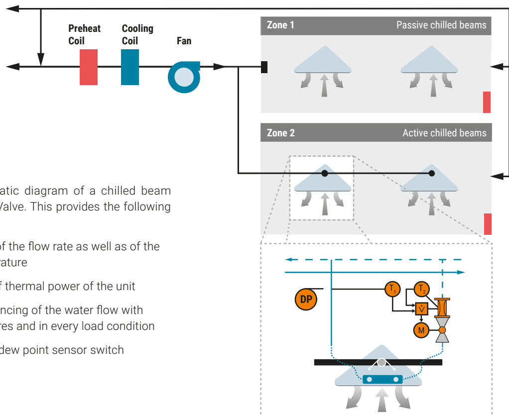
Abb. 84: Chilled beams in a multi-zone system.
