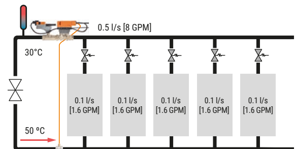
Abb. 103: With a Belimo Energy Valve™, the flow in the branch can be measured when each valve is opened, allowing verification.
