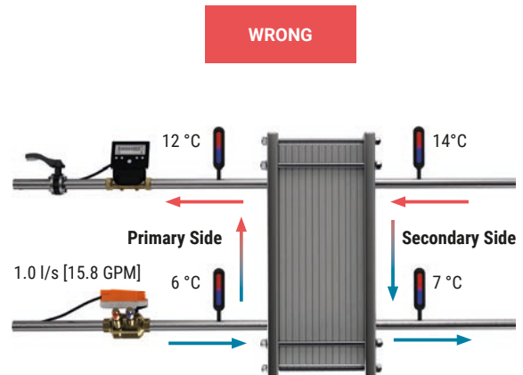
Abb. 70: Dynamic balancing.
