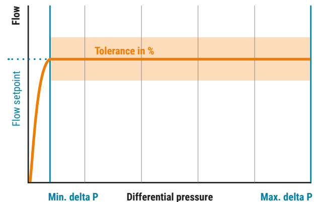
Abb. 50: Dynamic balancing ensures an accurate flow rate.
