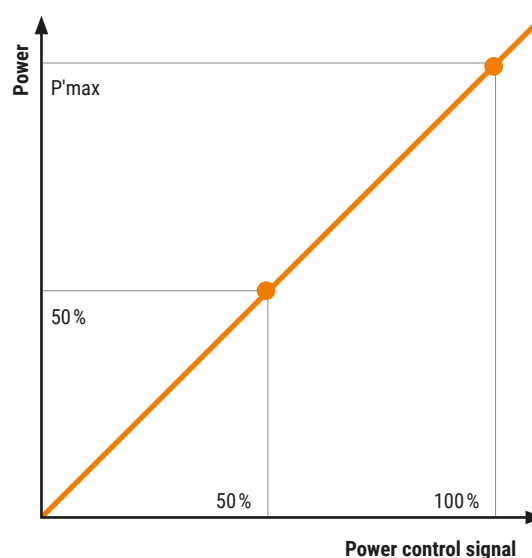
Abb. 26: Control characteristics in power control mode.
