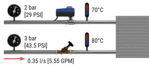
Abb. 97: FCU in heating mode.
