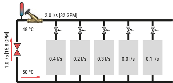
Abb. 104: An accidentally opened bypass valve may be discovered only after weeks, months or even years.
