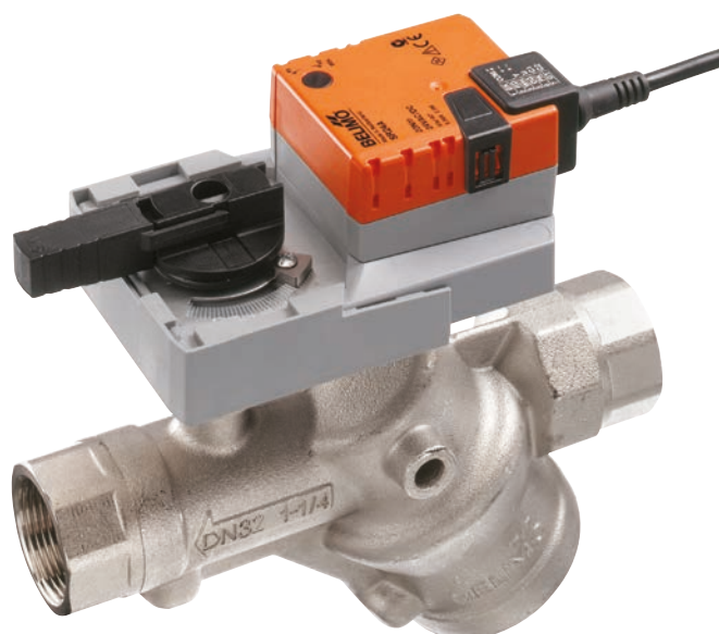
Abb. 8: PICCV, the first Belimo pressure-independent valve.
