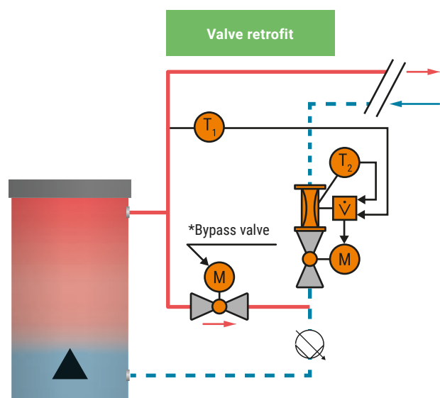
Abb. 117: A non-condensing boiler retrofitted with an air-bubbletight bypass valve and an Energy Valve.
