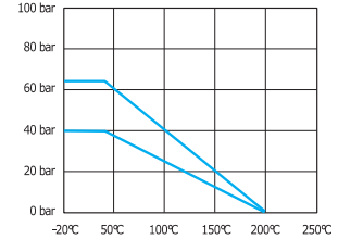
Pressure-temperature diagram
