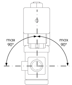
Maximum angle 90°.
