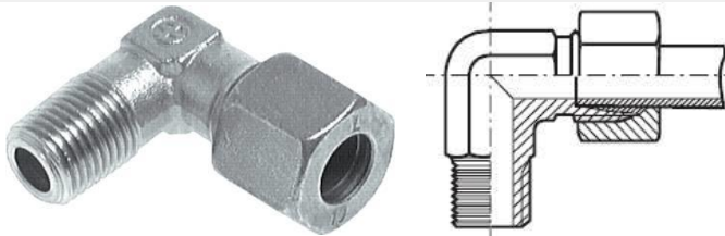
Angle screw in connections (R-threads / G-threads)
