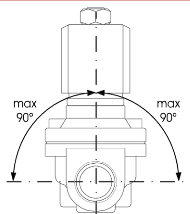
Maximum angle 90°.
