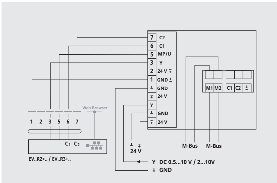
G-22PEM-A01 / M-Bus / EV..R2+.. / EV..R3+..
