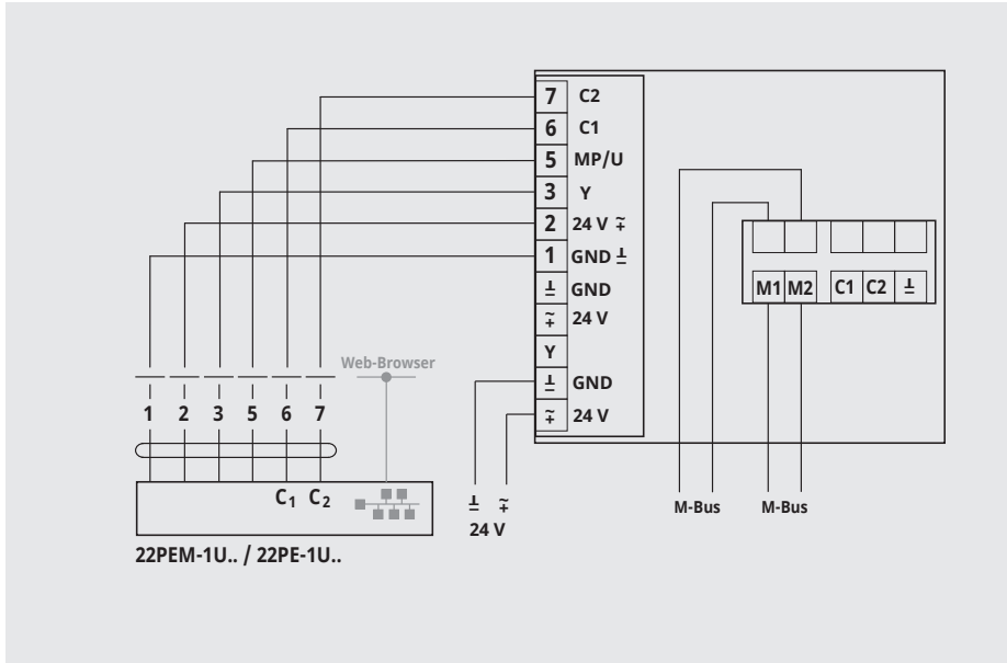
G-22PEM-A01 / M-Bus / 22PEM-1U.. / 22PE-1U..
