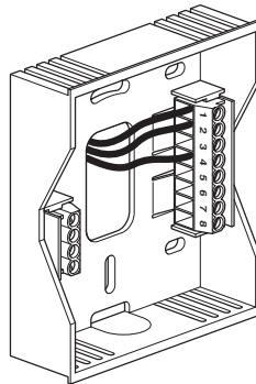
Flush-mounted connection
