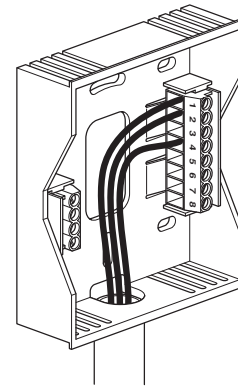
Surface-mounted connection
