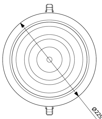
LEDDownlightRc-P-MW R200
