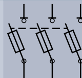
3-pole switchable
