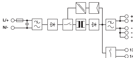
Block diagram
