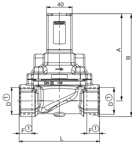
Threaded version DN32, 50
