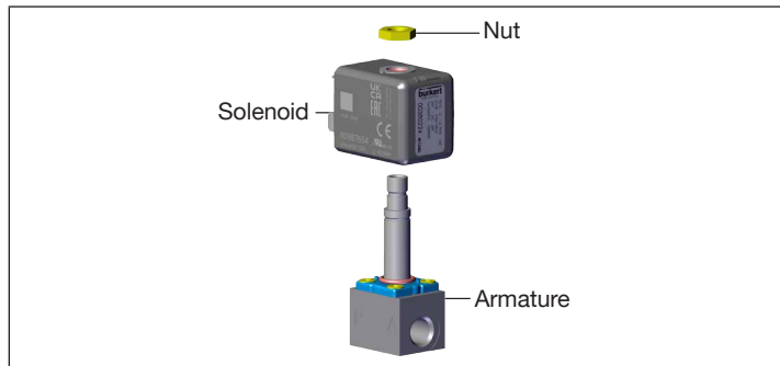
Fig. 6: Spare parts
