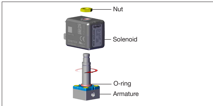
Fig. 5: Rotating the solenoid
