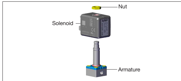
Fig. 6: Spare parts
