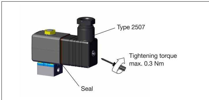
Fig. 4: Electrical connection
